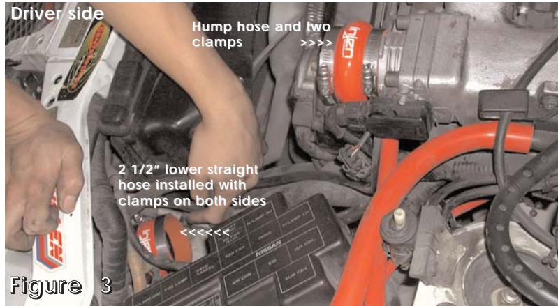
The 2 1/2" straight hose and hump hose have replaced the stock air intake ducts.
