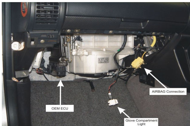
Figure 2 – Left hand footwell showing glove compartment removed
